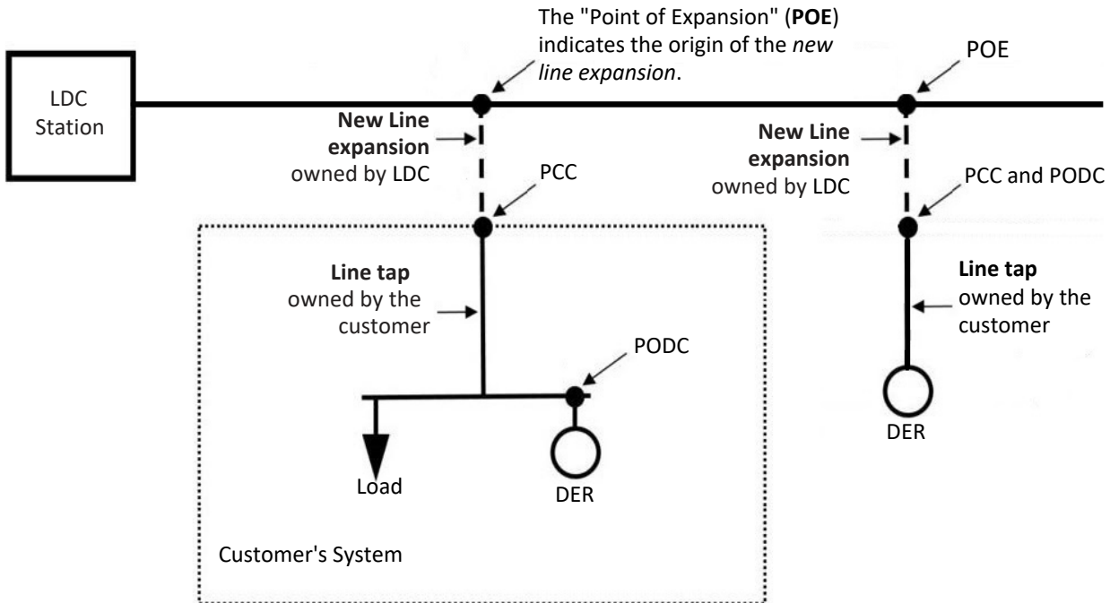
Figure A2: Where There is a New Renfrew Hydro Owned Line Expansion
