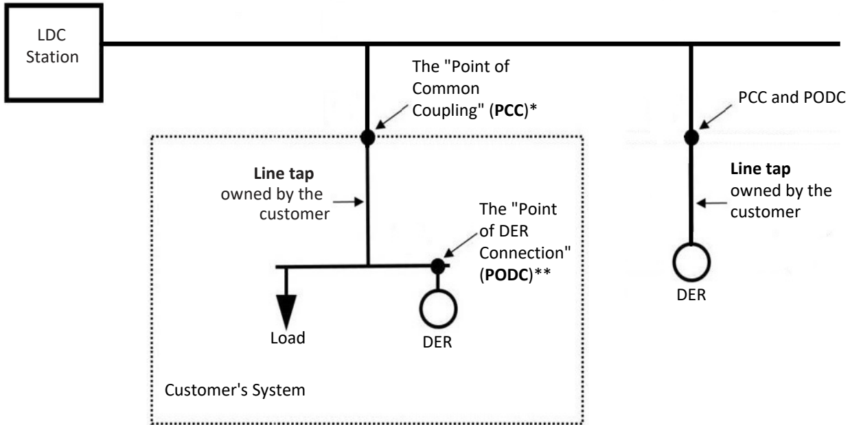
Figure A1: Where There is No New Renfrew Hydro Owned Line Expansion
